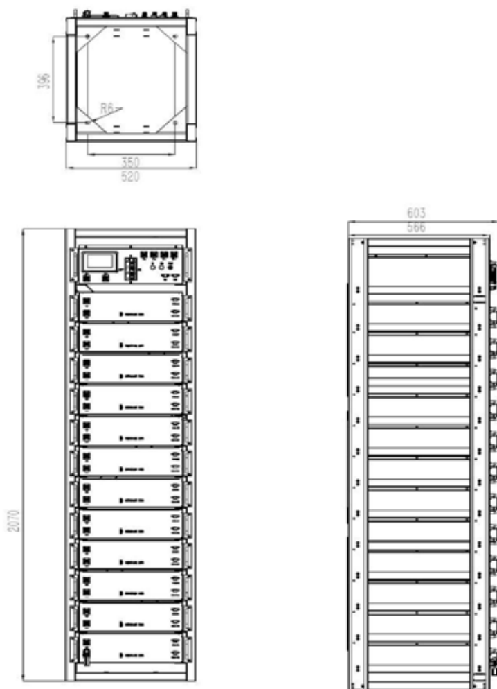
Fig. 3-3 FU60-RH Cluster dimension drawing-2
