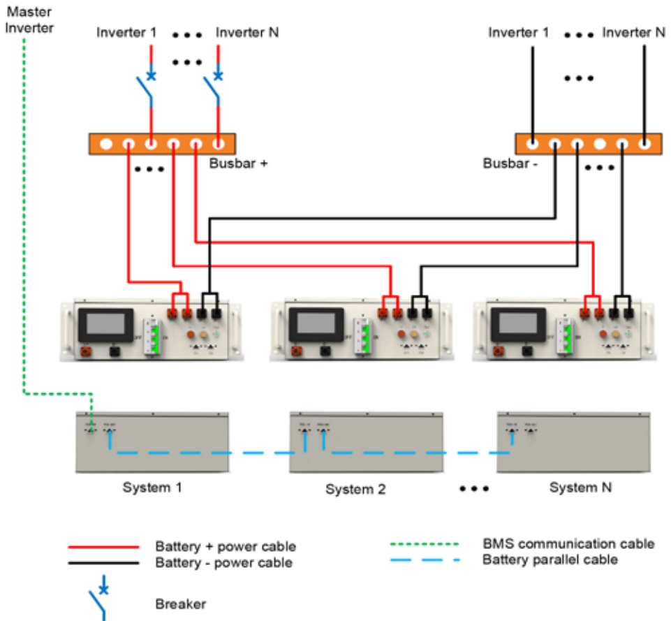
Fig. 4-2 FU30/35/40/45/50/55/60-RH +multi inverter diagram
