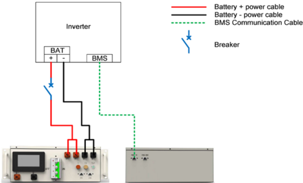
Fig. 4-1 FU30/35/40/45/50/55/60-RH single inverter diagram
