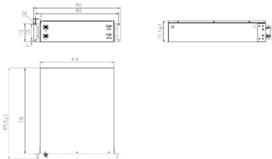
Fig. 3-2FU5-RH PACK dimension drawing-1
